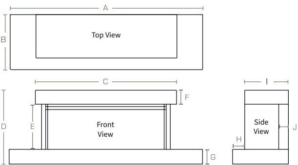
Brockenhurst 1200
