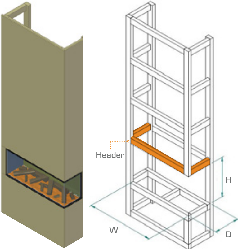
Two-sided installation
