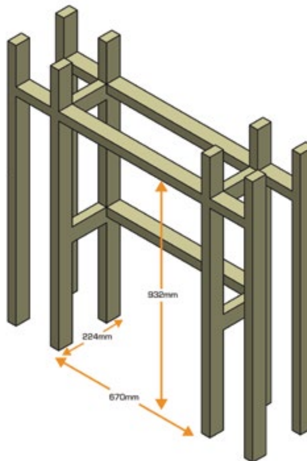
Open Dimensions for NF650sq Studwall Installation
