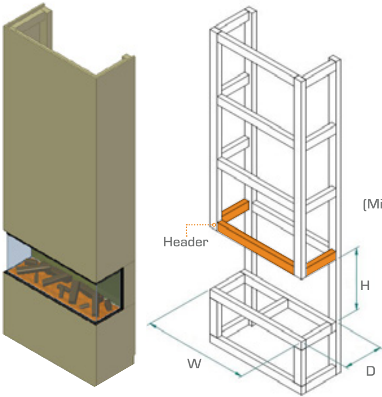
Three-sided installation
