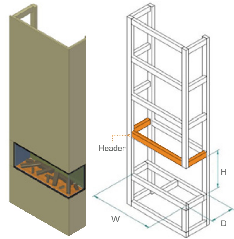
Two-sided installation
