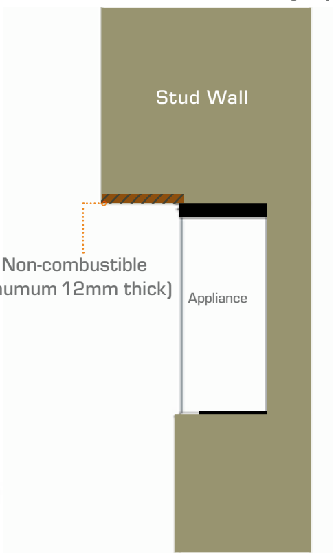
1200, 1600 & 1900 Non-Combustible Overhang Requirements
